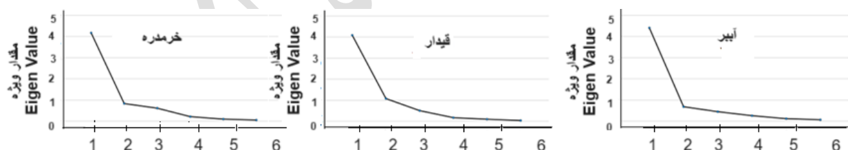
Figure 3. Screeplots of the selected stations (from left to right: Khorramdareh, Gheidar, and Abbar).
