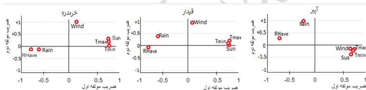
Figure 4. Geometrical positions of variables based on the first two factors in the selected stations (from left to right: Khorramdareh, Gheidar, and Abbar)
