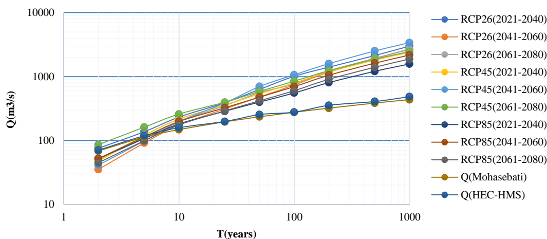
Figure 9. Flood esitimated in different return periods under climate change scenarios (2021-2080) for Whole Nazlu basin in comparison with historical recorded and modeled results
