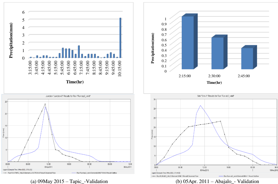
Figure 6. The simulated hydrograph (blue curve) compared to observations (black curve)
