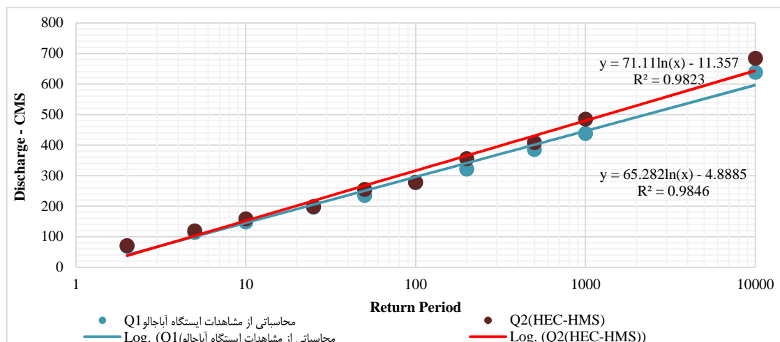
Figure 7. The comparison of peak discharge calculated with Lognormal distribution (Q1) and HEC-HMS simulated peak discharge (Q2) at Abajalu station in Different Return periods
