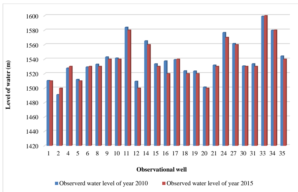
Figure 4. Water levels in observation wells at the first and fifth-year time steps
