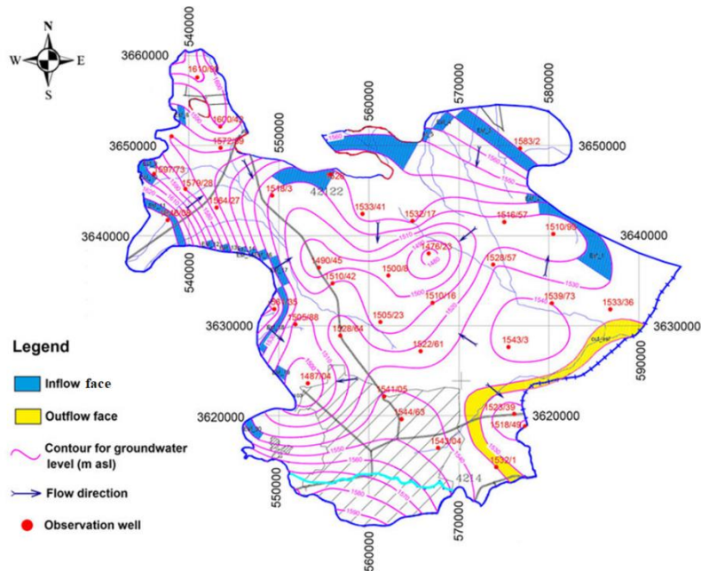
Figure 2. Groundwater potentiometric map of the Isfahan-Borkhar aquifer
