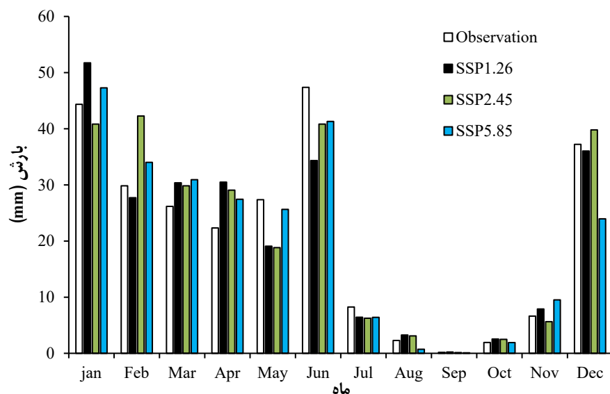
Figure 5. precipitation changes under different scenarios in the future (2026-2045)
