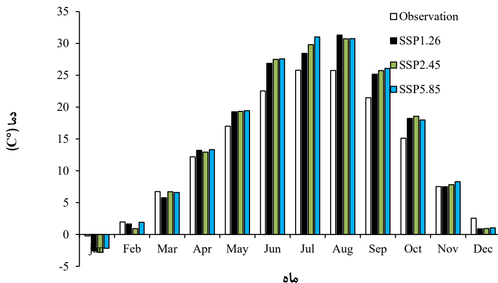
Figure 4. Temperature changes under different scenarios in the future (2026-2045)
