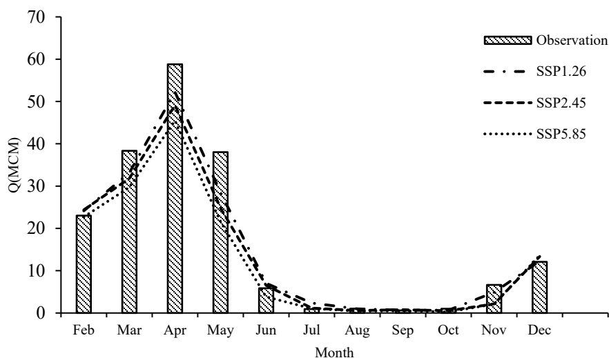
Figure 10. Changes in flow rate under different scenarios in the future (2026-2045).
