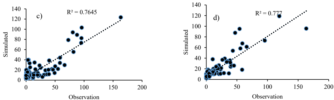
Figure 8. Scatter plot of observed and simulated test data around the regression line using ANN and ANN-PSO models. a) Scenario (1) ANN- b) Scenario (2) ANN- c) Scenario (1) ANN-PSO - d) Scenario (2) ANN-PS.
