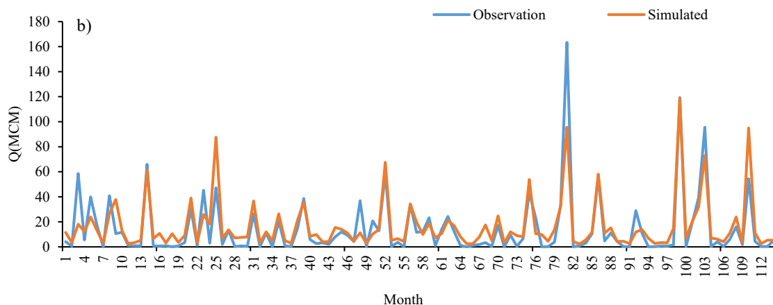
Figure 7. Time series diagram of observed and simulated test data using ANN-PSO model. a) Scenario 1 b) Scenario 2.
