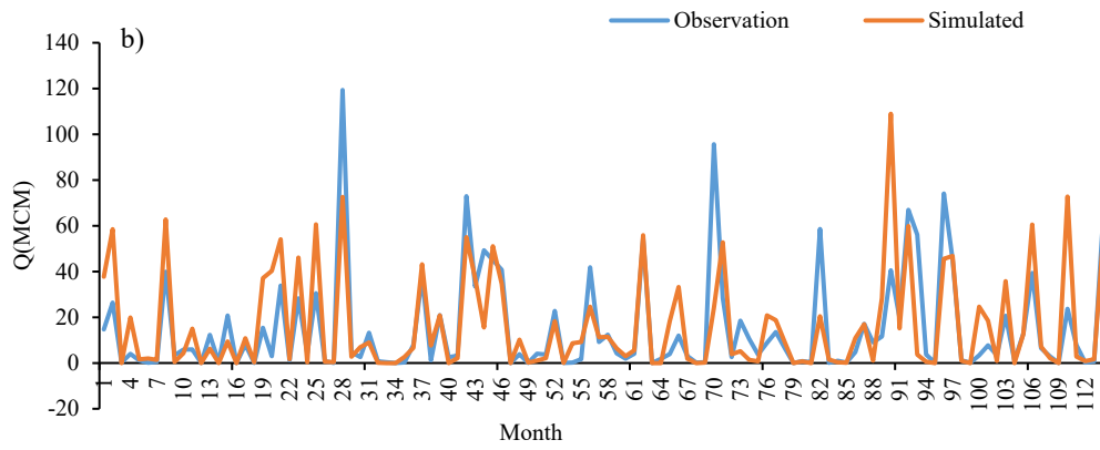
Figure 6. Time series diagram of observed and simulated test data using ANN model. a) Scenario 1 b) Scenario 2
