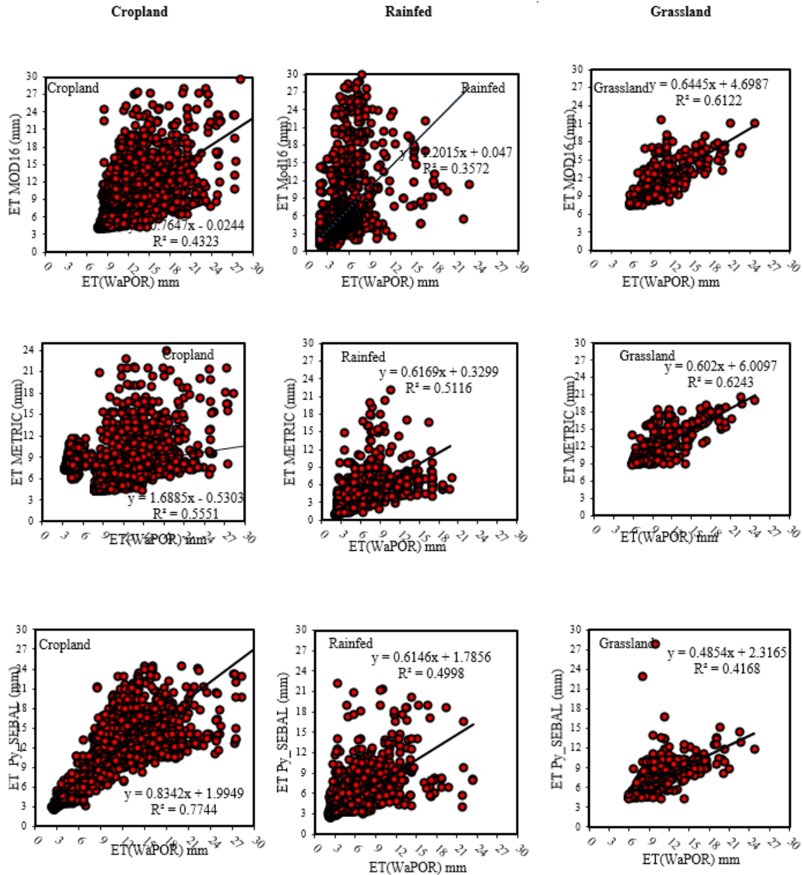
Figure 5. Comparison of evapotranspiration values obtained from the WaPOR model with evapotranspiration values derived from the Py_SEBAL, METRIC, and MOD16 models in three different land types
