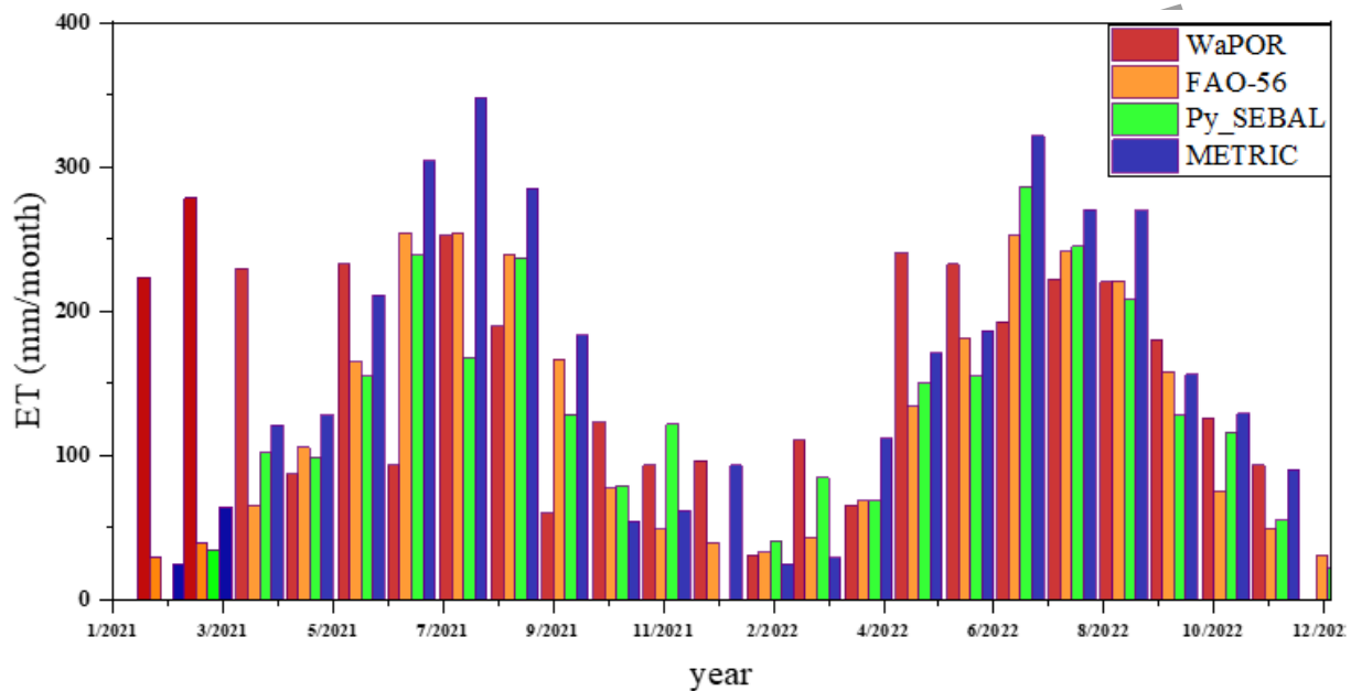
Figure 3. Estimated values of evapotranspiration by different models.
