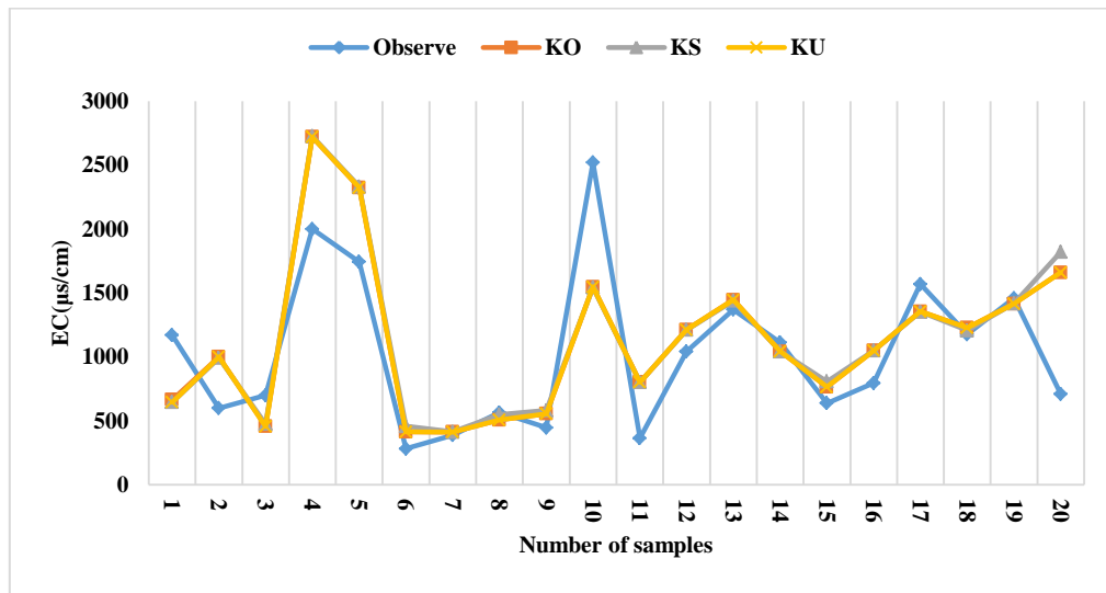
Figure 5. Evaluation of different EC parameter interpolation methods in the test phase
