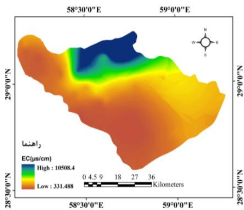
Figure 7. Spatial distribution of EC changes, ordinary kriging
