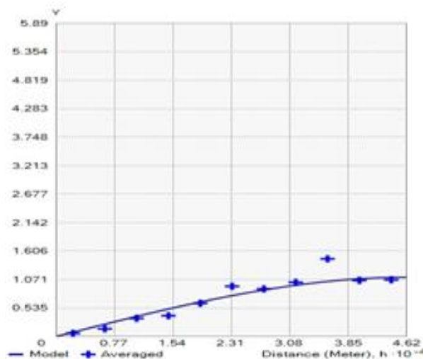
Figure 3. Experimental variable related to TDS parameter in OK method
