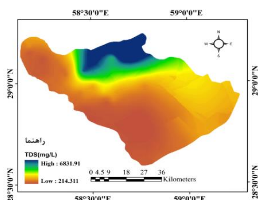
Figure 10. Spatial distribution of TDS changes, universal kriging
