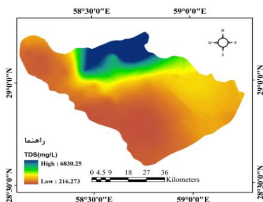
Figure 9. Spatial distribution of TDS changes, ordinary kriging
