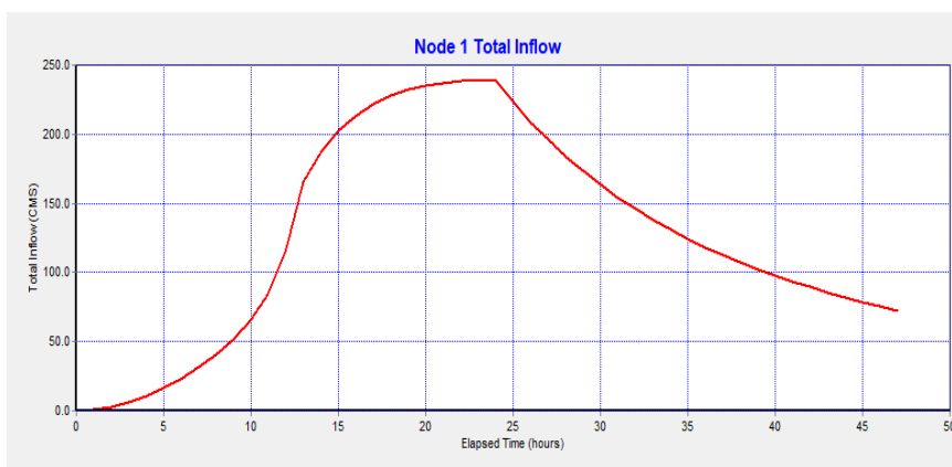
Figure 2. Hydrograph of Tajen basin outflow during the return period of five years
