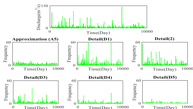
Figure 4. Wavelet decomposition of the observed Khoshkroud daily discharge time series with five levels using db7
