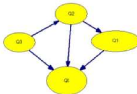
Figure 4. Conceptual model of BN model for M3 input pattern
