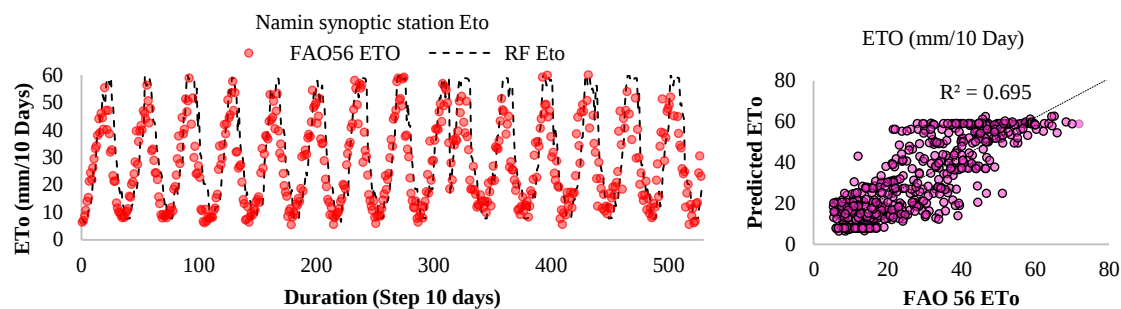
Figure 7. Estimated reference evapotranspiration for Namin station in RF method
