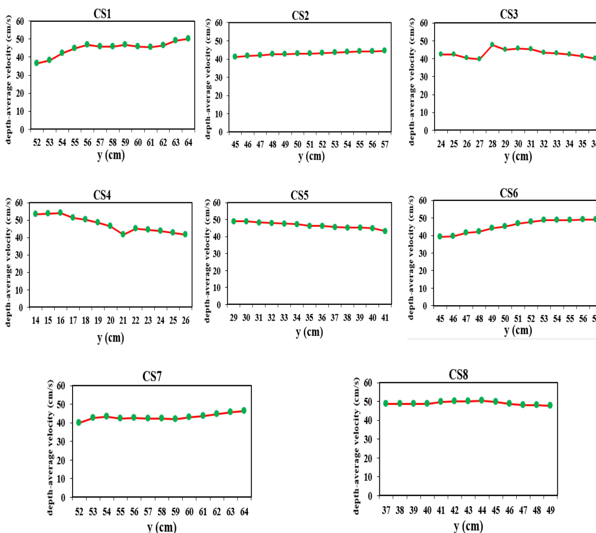
Figure 8. Depth average velocity distribution profiles at different sections and transverse direction for inbank flow ( D = 0.12 \text{ m} )
