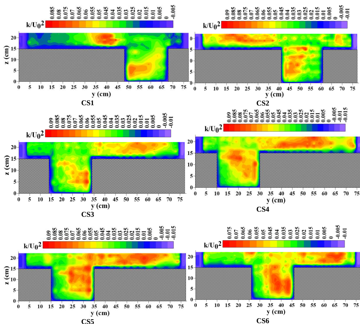
Figure 7. Turbulence kinetic energy contours at different sections of the meandering compound channel for overbank flow with a relative depth of 0.46
