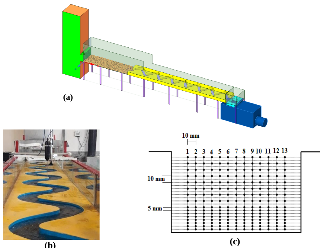
Figure 1. (a) A view of the laboratory channel with a compound meandering channel geometry (b) the flow in the main channel and the three-dimensional acoustic velocimeter (ADV) device and (c) the network of velocity measurement points in a section of the main channel
