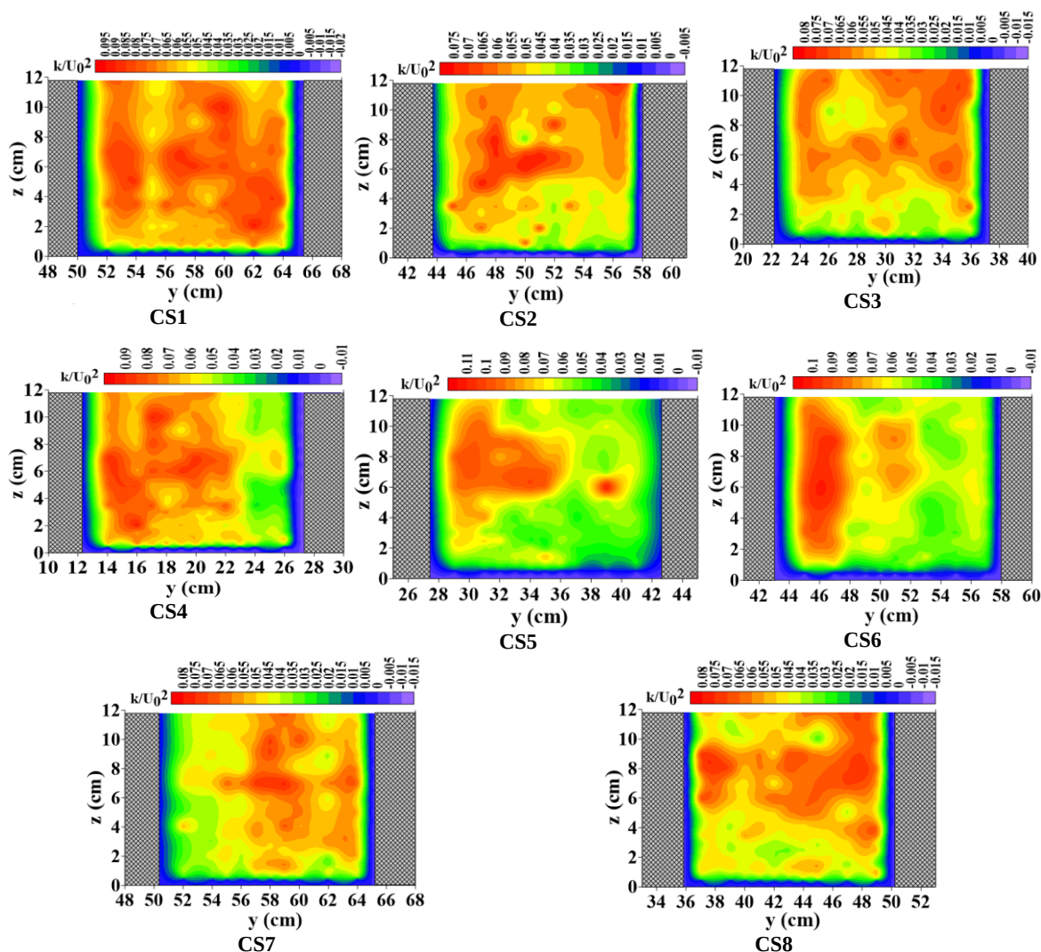
Figure 6. Turbulence kinetic energy contours in the main channel of compound meandering channel with depth of -0.12 m
