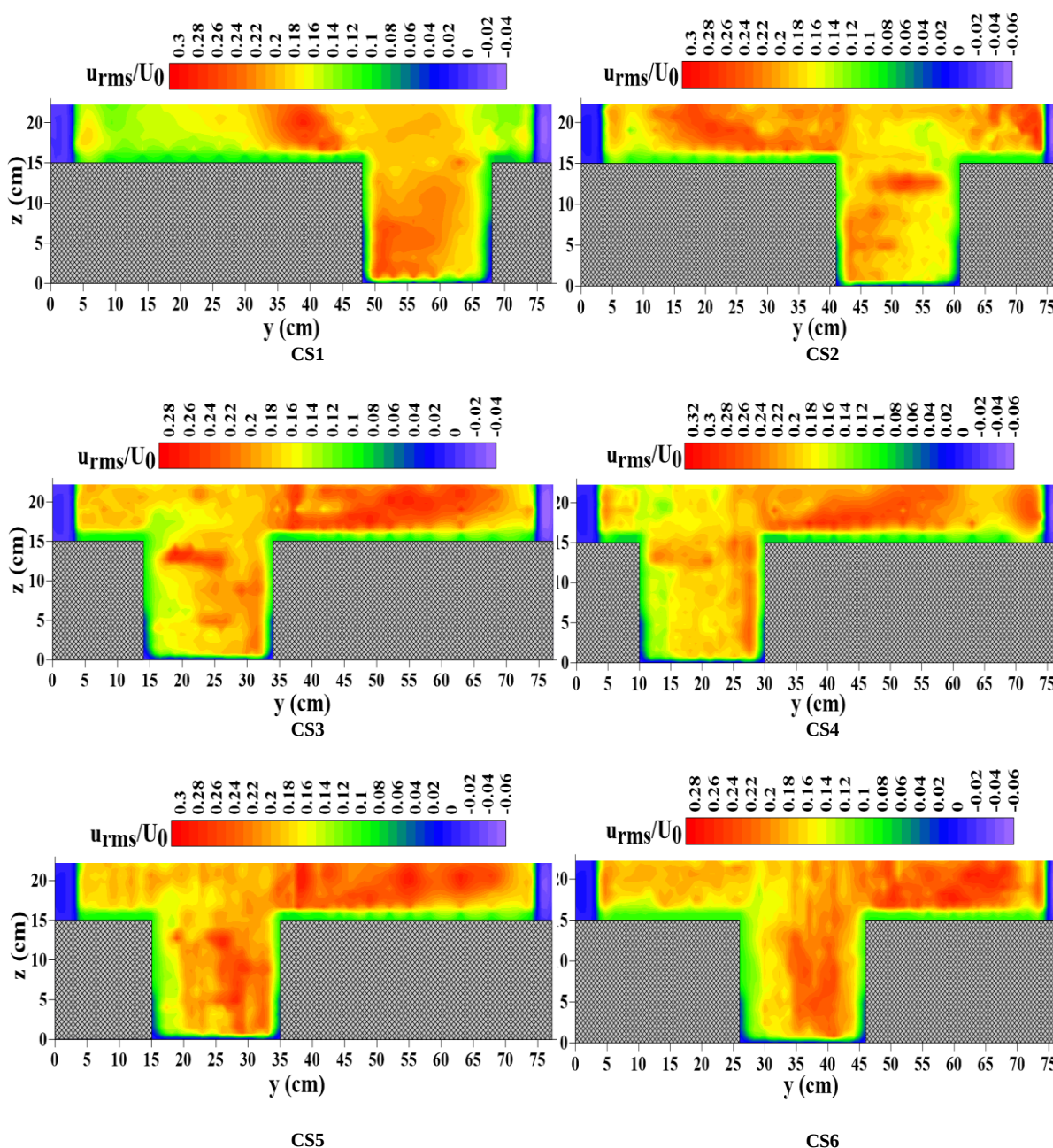
Figure 5. Longitudinal turbulence intensity contours in overbank flow at different sections with a relative depth of 0.46
