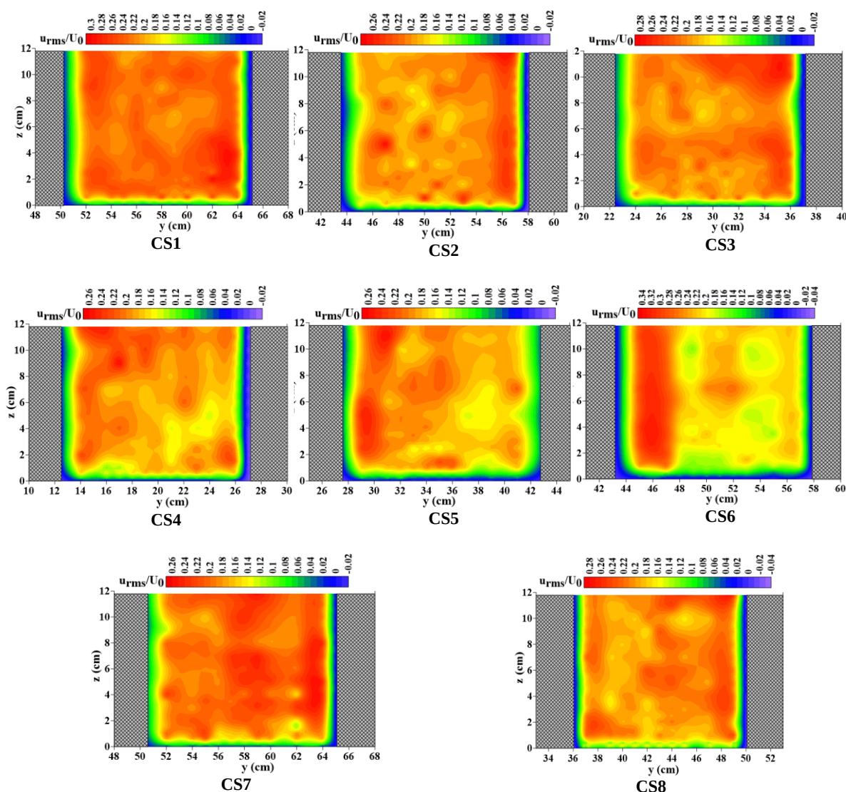
Figure 4. Longitudinal turbulence intensity contours at different sections of the main channel with a depth of 0.12 m
