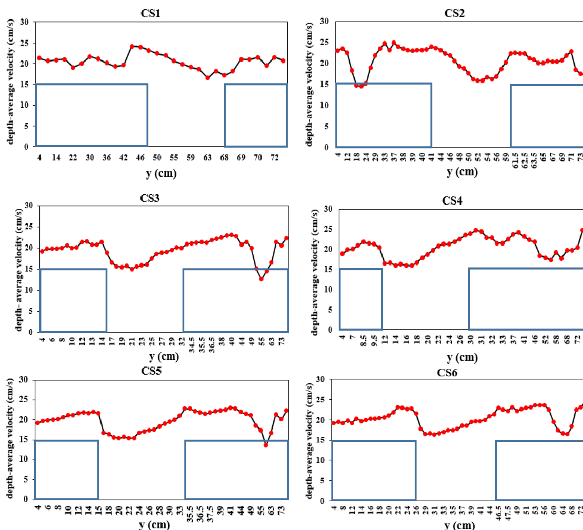
Figure 9. Depth average velocity distribution profiles at different sections and transverse direction for overbank flow ( D_r = 0.46 )
