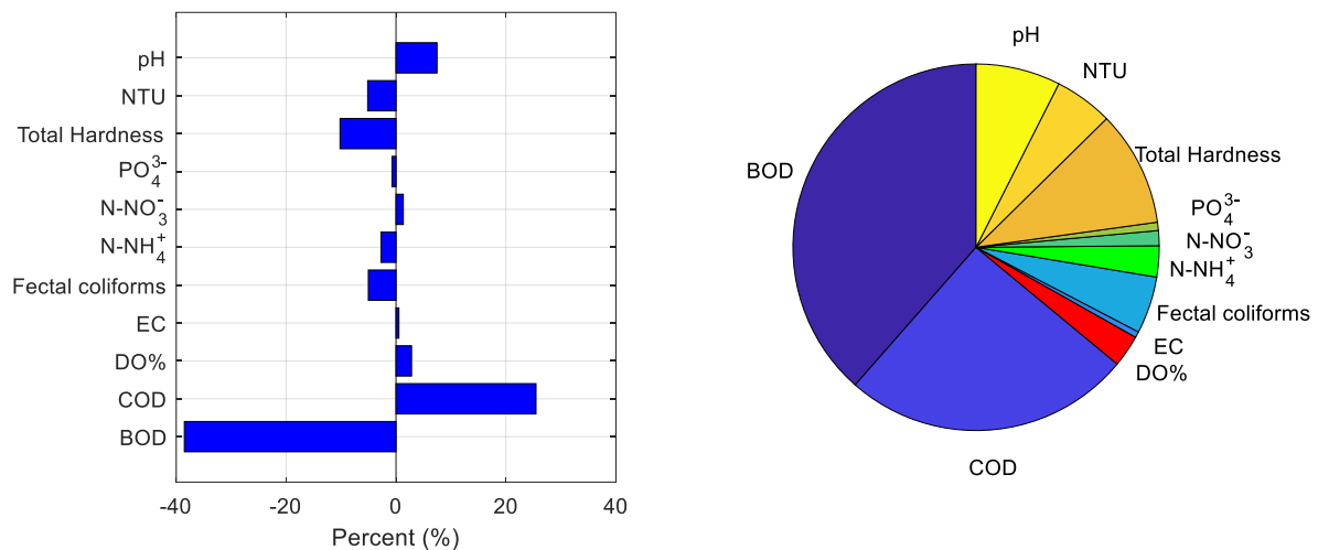
Figure 8. Parameter contributions to the water quality index during winter
