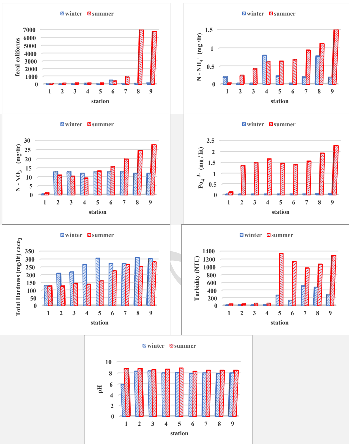
Figure 3. Variations of BOD 5 , COD, DO%, EC, Fecal Coliform, Ammonium, Nitrate, Phosphate, Total Hardness, Turbidity, and pH at 9 stations along the river during two sampling seasons (winter vs. summer)
