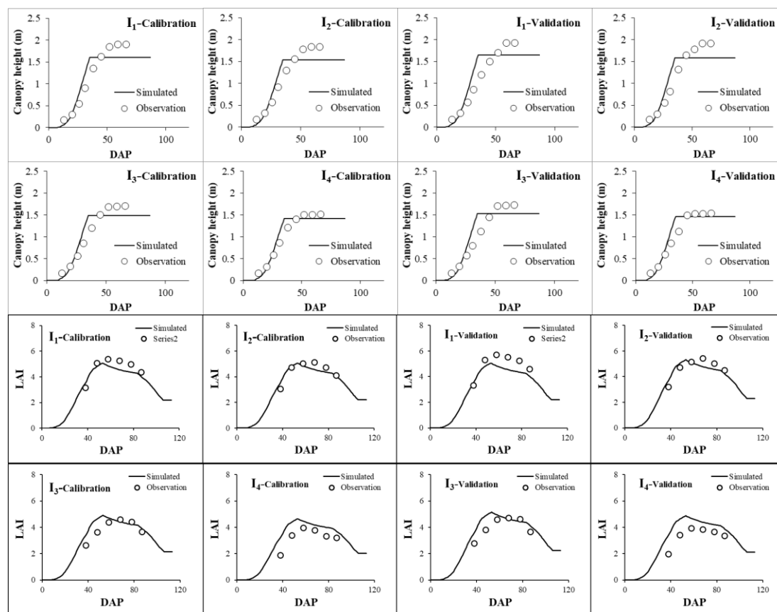
Figure 3. Calibration and validation of the measured and predicted values by the Ceres_Mazie model for the growth trend of sweet corn leaf area index (LAI) and canopy height at different irrigation levels for day after planting (DAP)
