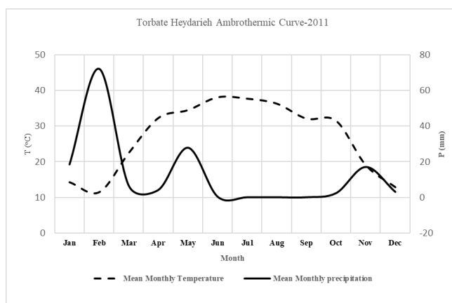
Figure 3. The ambrothermic curve of Torbat Heydarieh Hydroclimatology
