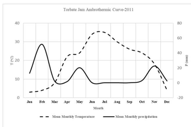
Figure 2. The ambrothermic curve of Turbate Jam climatology station
