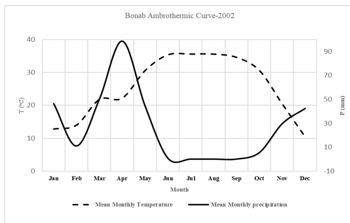
Figure 6. The ambrothermic curve of Bonab Hydroclimatology station
