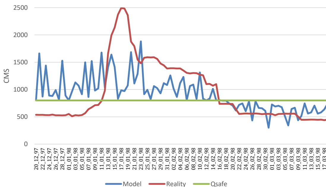
Figure 10. Reservoir release at a permissible discharge of 800 cubic meters per second
