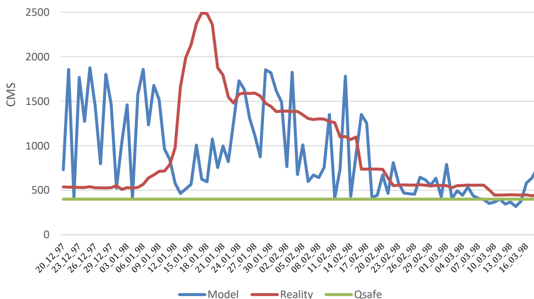
Figure 8. Reservoir release at a permissible discharge of 400 cubic meters per second
