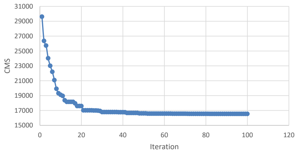
Figure 7. Convergence trend of the objective function for a permissible discharge of 800 CMS
