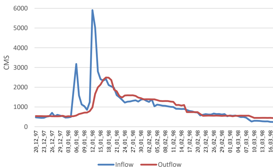
Figure 3. Inflow and outflow discharge from the Karkheh Dam reservoir
