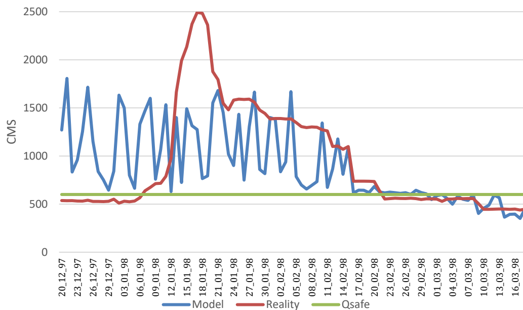
Figure 9. Reservoir release at a permissible discharge of 600 cubic meters per second
