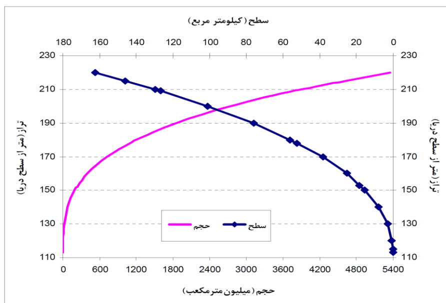
Figure 2. Reservoir volume-elevation curve of Karkheh Dam
